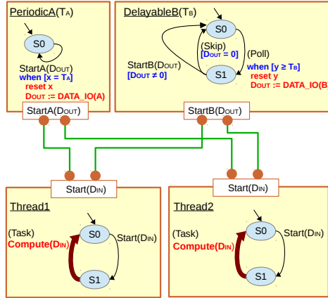
Figure 4: BIP model example
