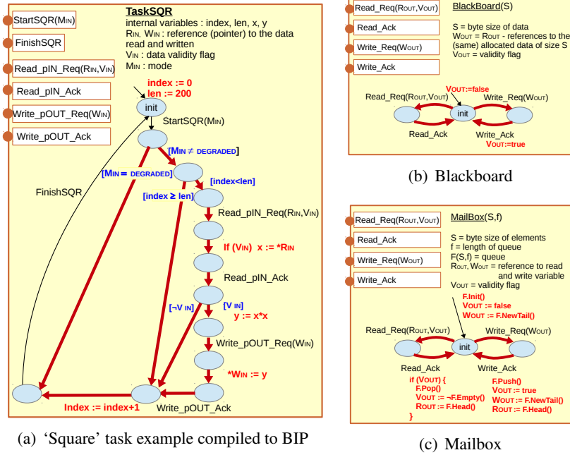
Figure 9: Compiling Tasks and Data Channels to BIP
