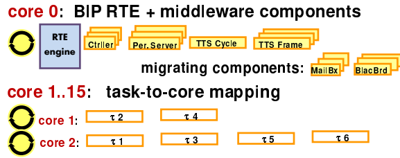
Figure 11: BIP Software Model and its Deployment on Multi-Core System
