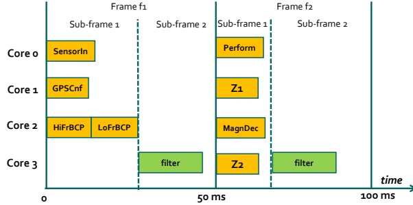
Figure 13: Optimized Static TTS Schedule for the FMS sub-system
