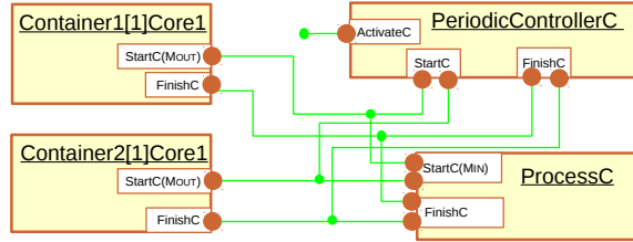
Figure 10: Connection between a Periodic Task and its Containers
