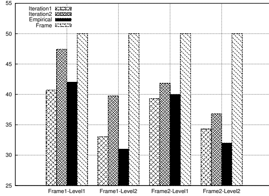
Figure 14: Worst-case finish time [ms] of last sub-frame in each TTS frame as computed at ‘Iteration 1’, ‘Iteration 2’, and empirically
