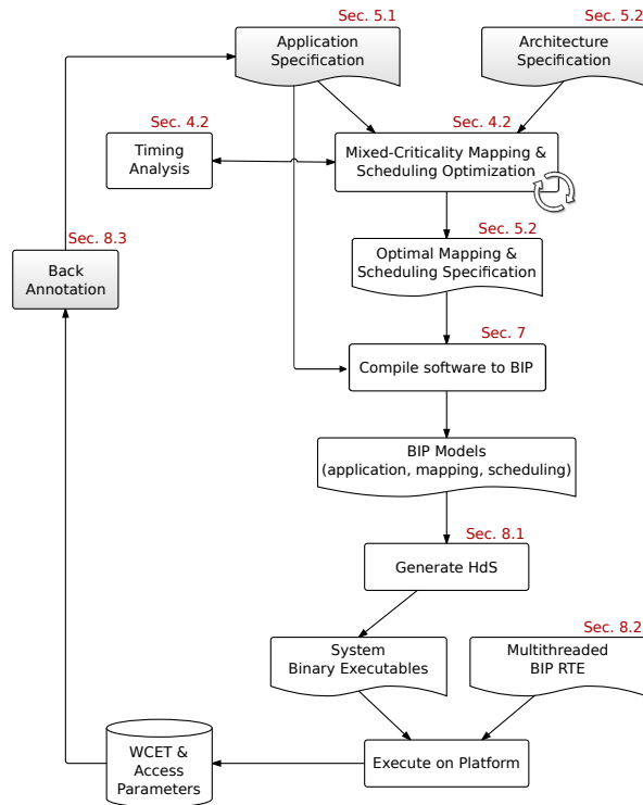
Figure 1: DOL-BIP-Critical Design Flow
