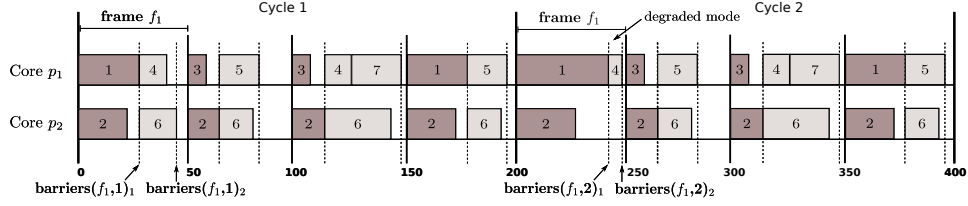
Figure 2: Global TTS schedule for 2 cycles (dark annotation: CL 2, light: CL 1)
