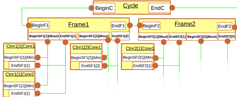
Figure 8: Composing Cycle, Frames and Containers
