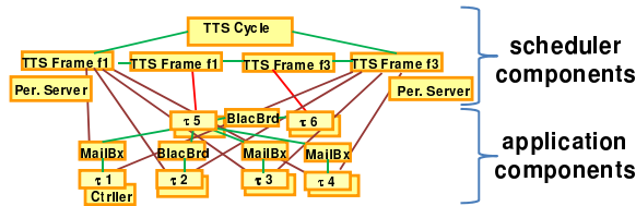
Figure 6: Overall BIP Software Model Obtained by Compilation from DOL-Critical
