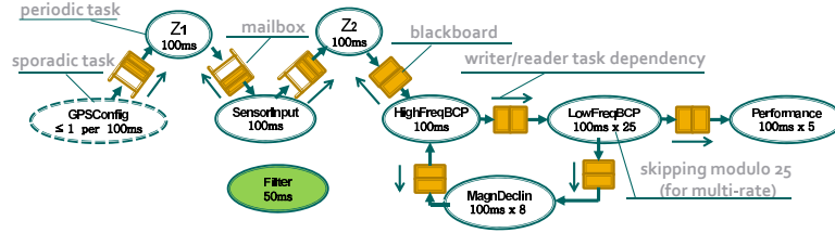
Figure 12: Flight Management System Test Case
