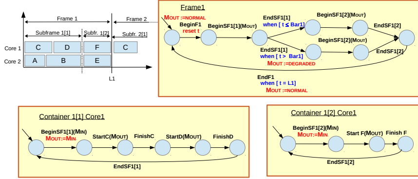
Figure 7: TTS Scheduling Frames in BIP
